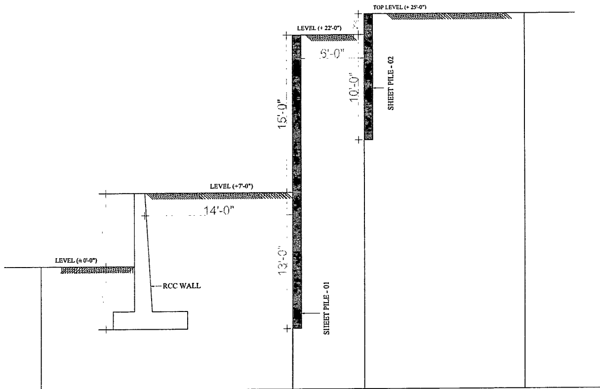
FIG: SITE PROTECTION ELEVATION
