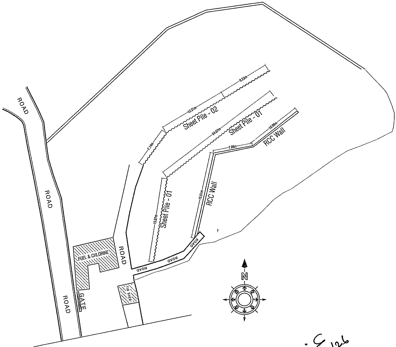
FIG: SITE LAYOUT PLAN OF WDZ 26.01
