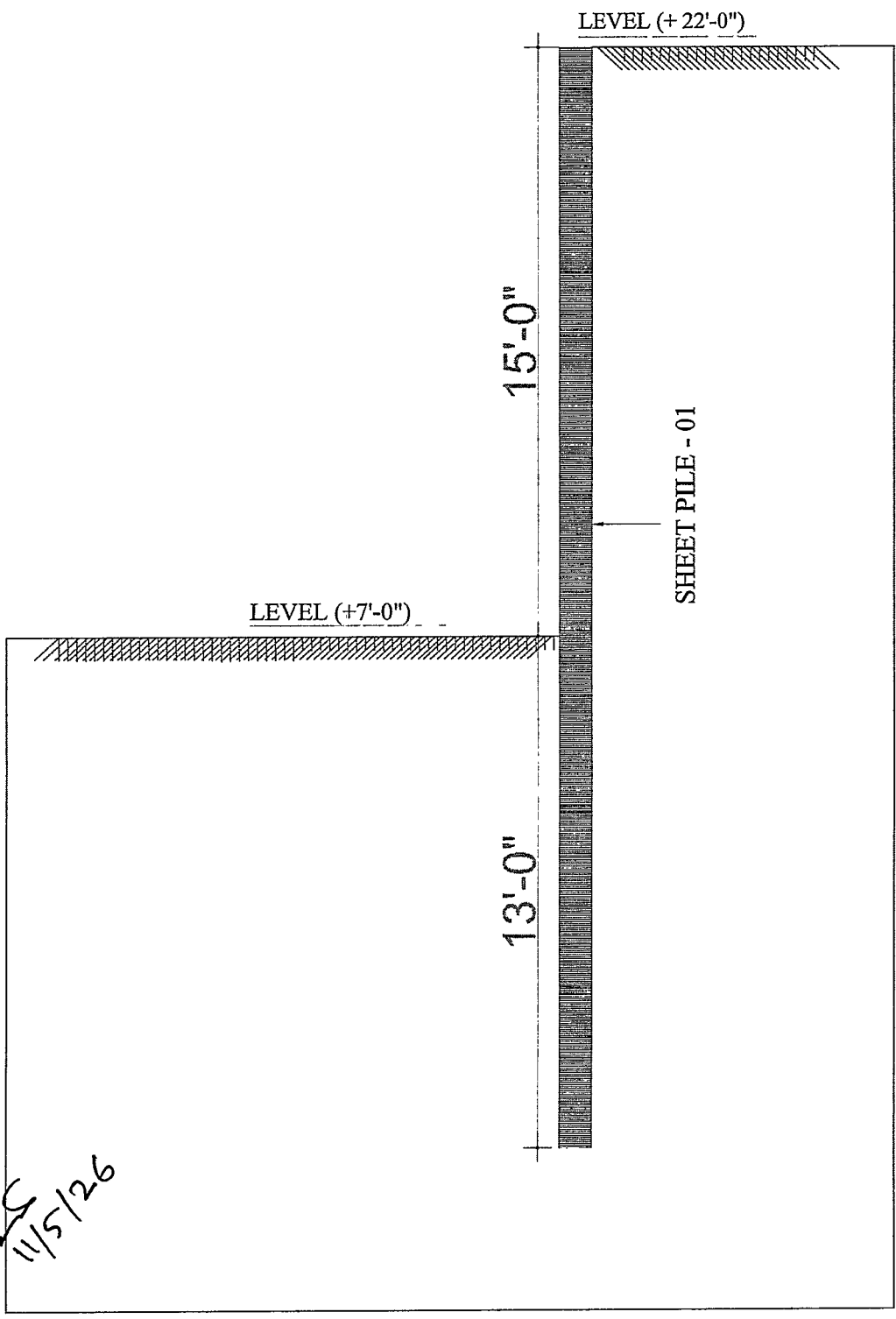
FIG: SHEET PILE -01 ELEVATION
