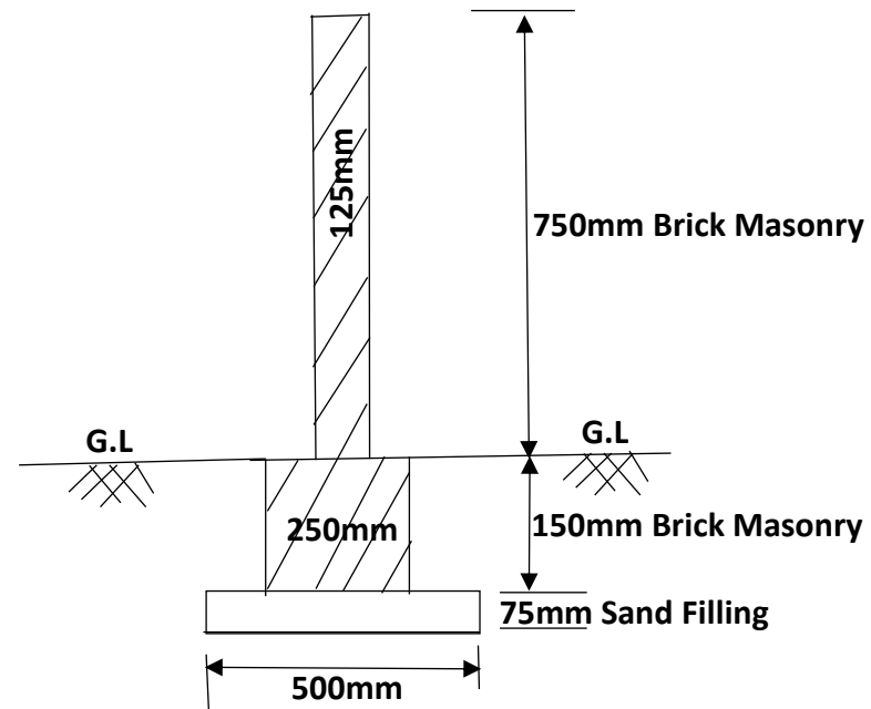
Drawing "Section A-A"
